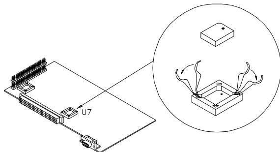
Figure 6. Removing the U7 Chip from the Socket
