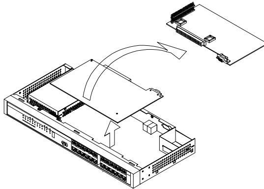
Figure 5. Removing the Board
