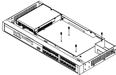
Figure 11. Replacing the Upper Board
