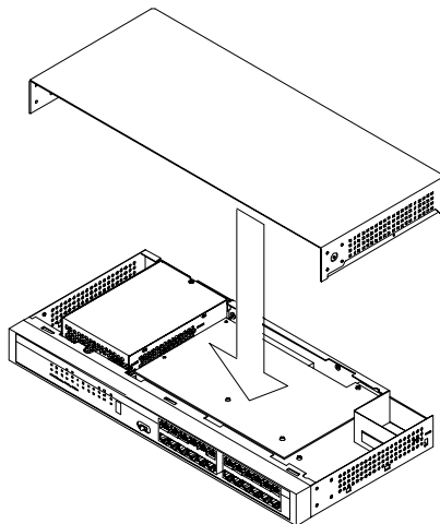
Figure 12. Replacing the Top Panel
