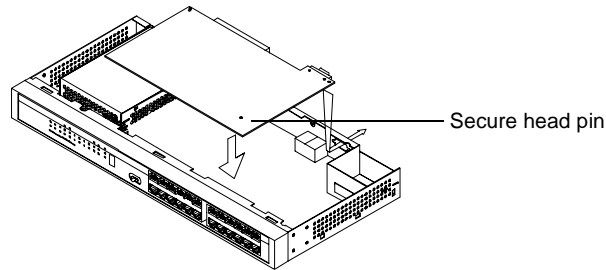
Figure 8. Replacing the Upper Board
