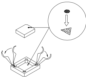
Figure 7. Aligning the Chip in the Socket
