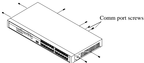
Figure 2. Exterior Screw Locations
