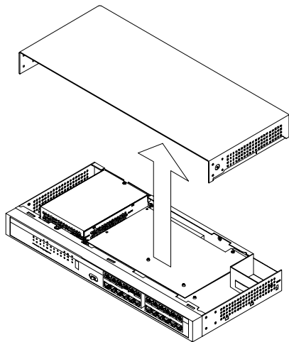
Figure 3. Removing the Top Panel
